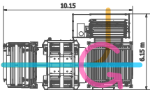
01 Rotating, Folding, 90° and Straight Transfer Operations on a single station
